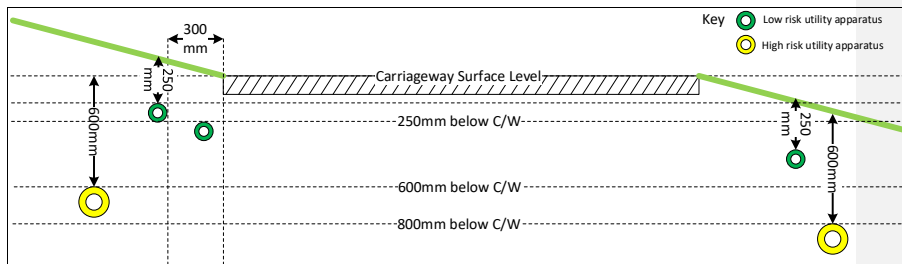
Figure 3 - Verge Datum Point no Interjoining Footway
