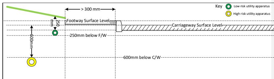
Figure 4 – Verge Datum Point with Interjoining Footway
