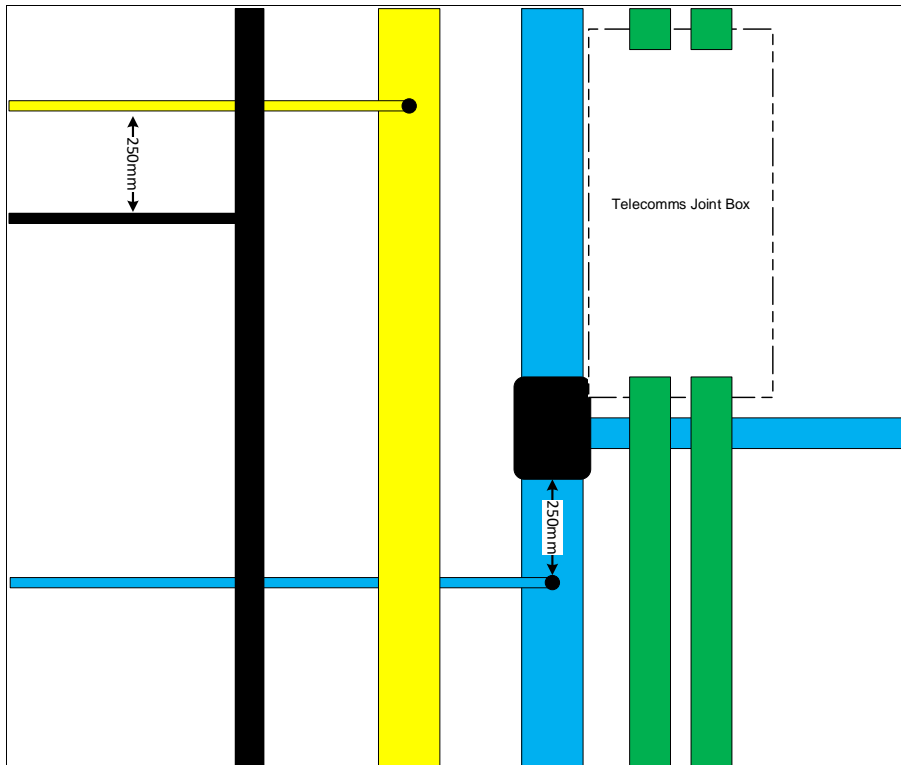
Figure 2 - Service Connection Point Lateral Proximity (Top-down Perspective)
