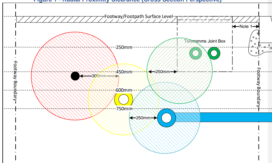
Figure 1 - Radial Proximity Clearance (Cross Section Perspective)
